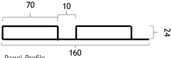
Panel Profile
