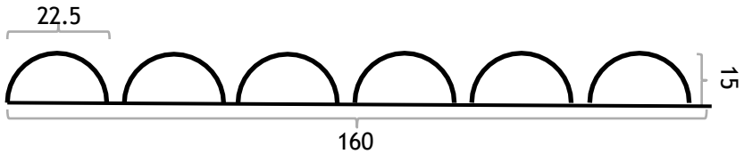
Panel Profile **Images are not to scale and are provided for illustrative purposes only. -Product sizes may vary depending on the manufacturing batch and year of manufacture. Please confirm the required dimensions with the supplier before placing your order.
