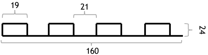
Panel Profile
