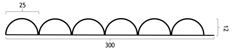
Panel Profile
