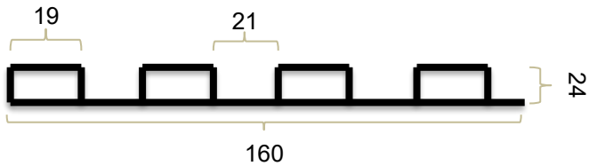
Panel Profile
