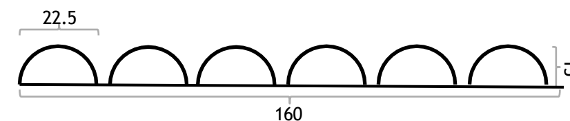
Panel Profile
