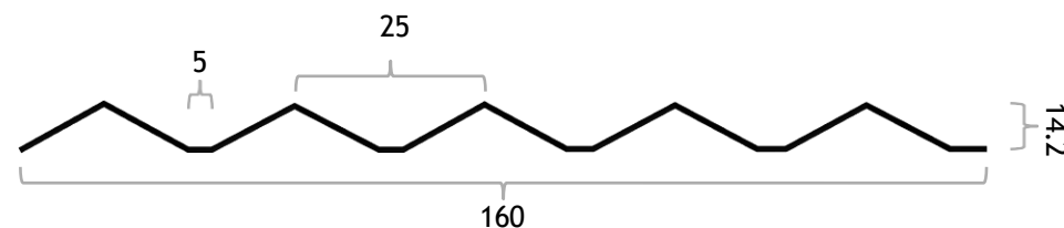
Panel Profile
