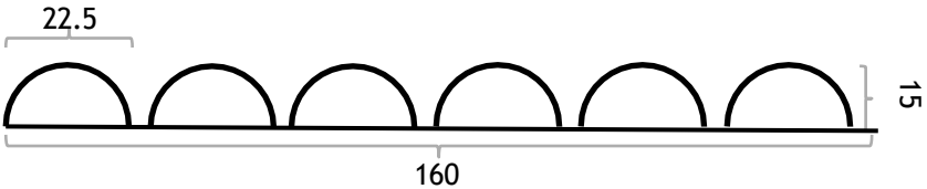
Panel Profile **Images are not to scale and are provided for illustrative purposes only. -Product sizes may vary depending on the manufacturing batch and year of manufacture. Please confirm the required dimensions with the supplier before placing your order.
