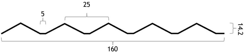
Panel Profile
