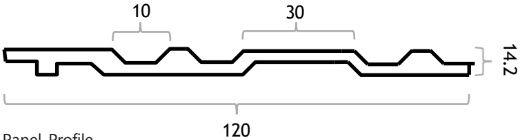
Panel Profile
