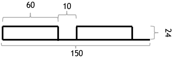
Panel Profile
