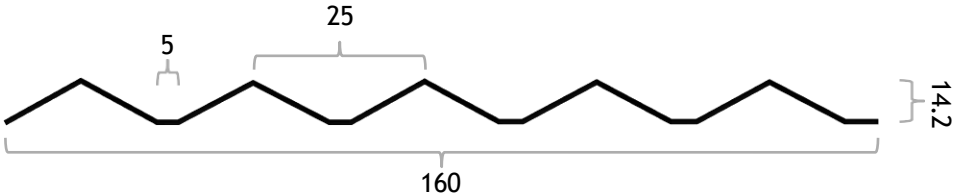
Panel Profile
