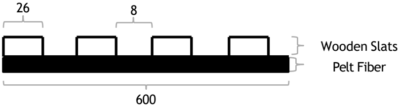
Panel Profile **Images are not to scale and are provided for illustrative purposes only. *Product sizes may vary depending on the manufacturing batch and year of manufacture. Please confirm the required dimensions with the supplier before placing your order.
