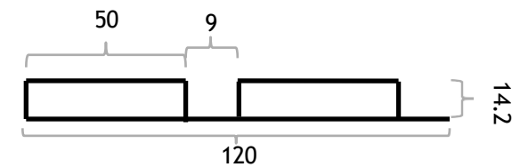
Panel Profile
