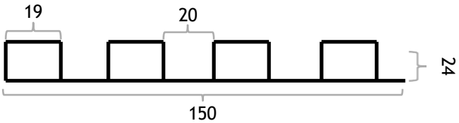
Panel Profile
